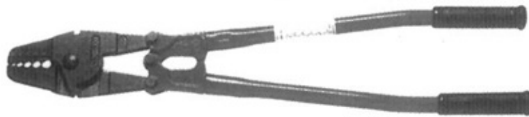
MODEL HSC-350 SWAGES 2mm TO 3,5mm ROPE MODEL HSC-600 SWAGES 2mm TO 5mm ROPE
